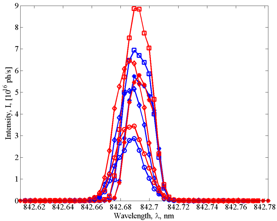
Figure 46. Spectra collected of the 842 nm line at all pressures.
