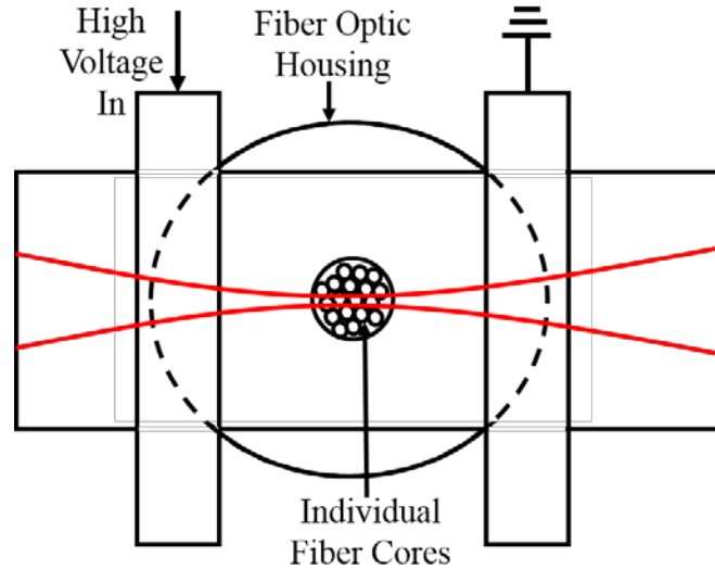
Figure 11. A visualization of the pump laser passing in front of the face of the fiber optic used during the OES experiment. Objects are not to scale as this figure was intended to increase understanding of the scenario introduced by Figure 10, not to portray the exact placement of the fiber optic or width of the pump laser as it passes through the test cell.
