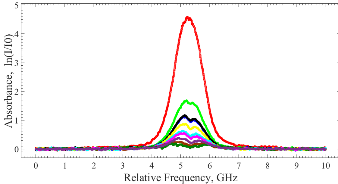
Figure 24. The absorption curves as a function of relative probe laser frequency for the data acquired when pressure inside the test cell was 5Torr. The red line is the absorption profile with only the scanning probe beam passing through the discharge (no pump beam). The various colors are the absorption profiles for different pump beam powers, light green for 10 mW, dark blue for 16 mW, black for 19 mW, yellow for 34 mW, cyan for 66 mW, magenta for 146 mW, purple for 231 mW, brown for 488 mW, and dark green for 899 mW.
