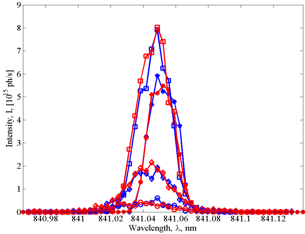
Figure 45. Spectra collected of the 841 nm line at all pressures.
